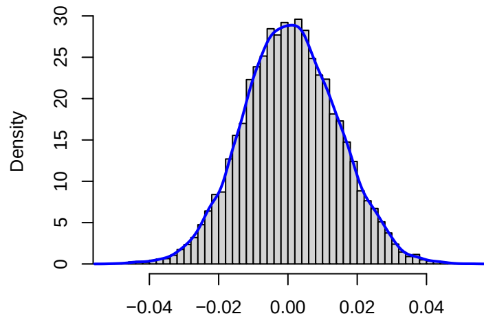
\theta_{1600,2}
