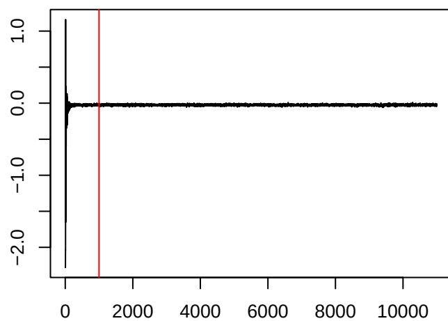
\theta_{800,2}
