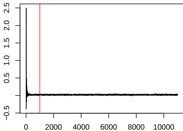
\theta_{400,2}
