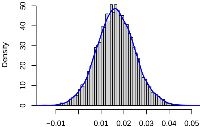
\theta_{1200,2}
