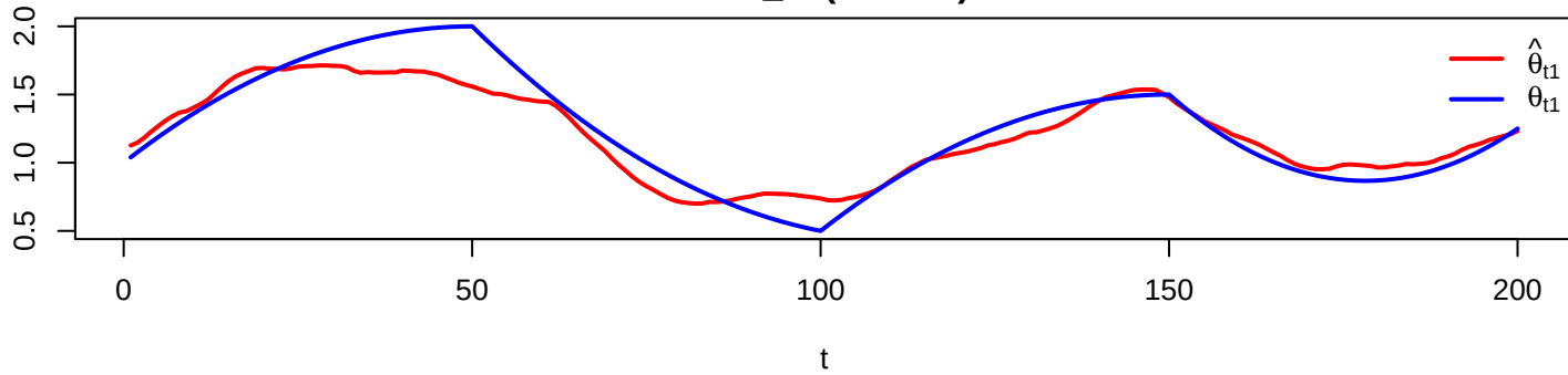
\theta_{t1} (chain 1)
