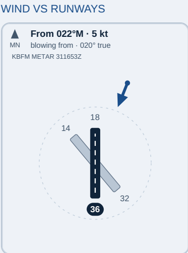
KBFM runway and wind diagram. Schematic: alignment only. Magnetic north is up. Runway length, width, relative position and intersections are not drawn and are not published in the runway table. Land runways drawn: 14/32, 18/36. Wind from 020 degrees true, 022 degrees magnetic, at 5 knots. Wind direction is the direction the wind blows FROM, so the arrow starts on the upwind side of the field and points across it. Wind-favoured runway end, highlighted: 36. Wind source: KBFM METAR 311653Z.
