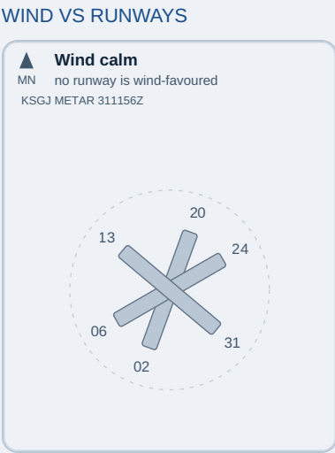
KSGJ runway and wind diagram. Schematic: alignment only. Magnetic north is up. Runway length, width, relative position and intersections are not drawn and are not published in the runway table. Land runways drawn: 13/31, 06/24, 02/20. Seaplane water lanes (17W, 35W, 18W, 36W, 12W and 30W) are excluded from the diagram and are never marked as favoured. Wind is calm, so no arrow is drawn and no runway is marked as favoured. Wind source: KSGJ METAR 311156Z.
