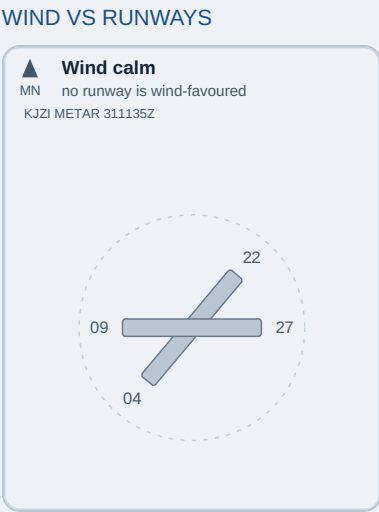
KJZI runway and wind diagram. Schematic: alignment only. Magnetic north is up. Runway length, width, relative position and intersections are not drawn and are not published in the runway table. Land runways drawn: 09/27, 04/22. Wind is calm, so no arrow is drawn and no runway is marked as favoured. Wind source: KJZI METAR 311135Z.
