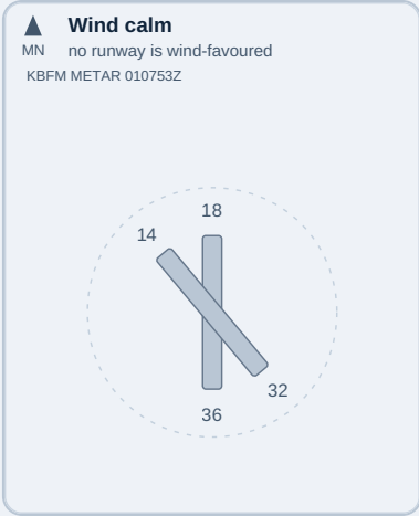
KBFM runway and wind diagram. Schematic: alignment only. Magnetic north is up. Runway length, width, relative position and intersections are not drawn and are not published in the runway table. Land runways drawn: 14/32, 18/36. Wind is calm, so no arrow is drawn and no runway is marked as favoured. Wind source: KBFM METAR 010753Z.
