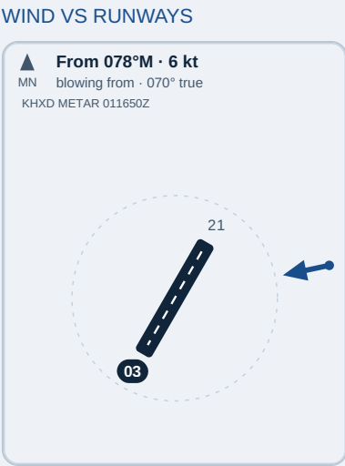
KHxD runway and wind diagram. Schematic: alignment only. Magnetic north is up. Runway length, width, relative position and intersections are not drawn and are not published in the runway table. Land runways drawn: 03/21. Wind from 070 degrees true, 078 degrees magnetic, at 6 knots. Wind direction is the direction the wind blows FROM, so the arrow starts on the upwind side of the field and points across it. Wind-favoured runway end, highlighted: 03. Wind source: KHxD METAR 011650Z.
