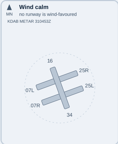
KDAB runway and wind diagram. Schematic: alignment only. Magnetic north is up. Runway length, width, relative position and intersections are not drawn and are not published in the runway table. Land runways drawn: 07L/25R, 16/34, 07R/25L. Wind is calm, so no arrow is drawn and no runway is marked as favoured. Wind source: KDAB METAR 310453Z.
