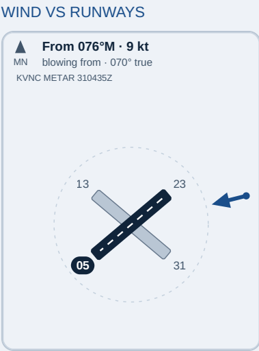
KVNC runway and wind diagram. Schematic: alignment only. Magnetic north is up. Runway length, width, relative position and intersections are not drawn and are not published in the runway table. Land runways drawn: 13/31, 05/23. Wind from 070 degrees true, 076 degrees magnetic, at 9 knots. Wind direction is the direction the wind blows FROM, so the arrow starts on the upwind side of the field and points across it. Wind-favoured runway end, highlighted: 05. Wind source: KVNC METAR 310435Z.
