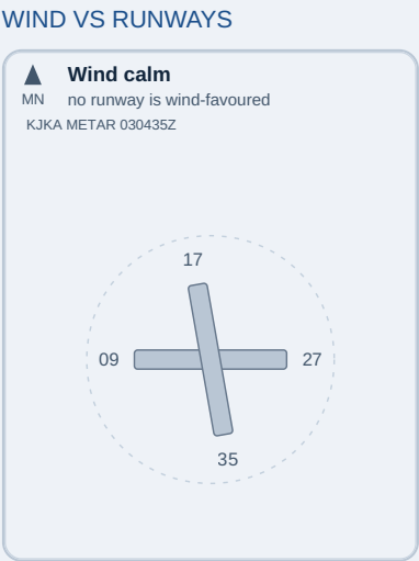
KJKA runway and wind diagram. Schematic: alignment only. Magnetic north is up. Runway length, width, relative position and intersections are not drawn and are not published in the runway table. Land runways drawn: 09/27, 17/35. Wind is calm, so no arrow is drawn and no runway is marked as favoured. Wind source: KJKA METAR 030435Z.
