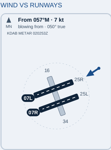
KDAB runway and wind diagram. Schematic: alignment only. Magnetic north is up. Runway length, width, relative position and intersections are not drawn and are not published in the runway table. Land runways drawn: 07L/25R, 16/34, 07R/25L. Wind from 050 degrees true, 057 degrees magnetic, at 7 knots. Wind direction is the direction the wind blows FROM, so the arrow starts on the upwind side of the field and points across it. Equally wind-favoured runway ends, highlighted: 07L and 07R. Wind source: KDAB METAR 020253Z.
