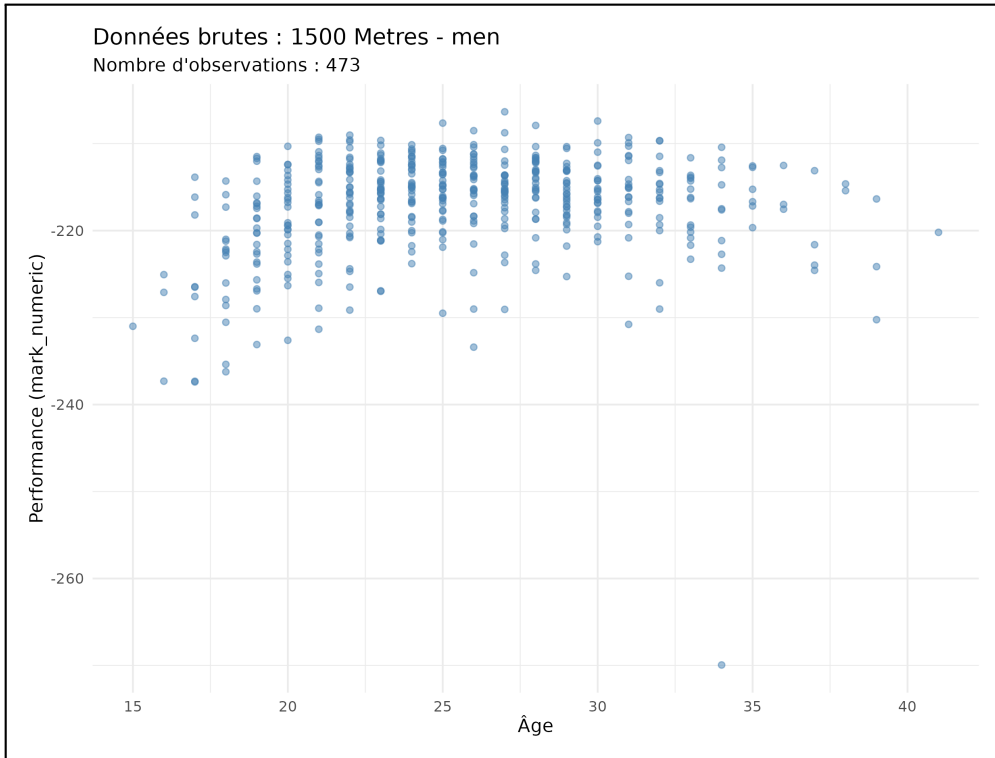
Figure 6: Top 32
