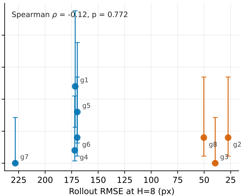
Planning success vs probe R^2 and vs rollout error (screening grid, seed 0)
