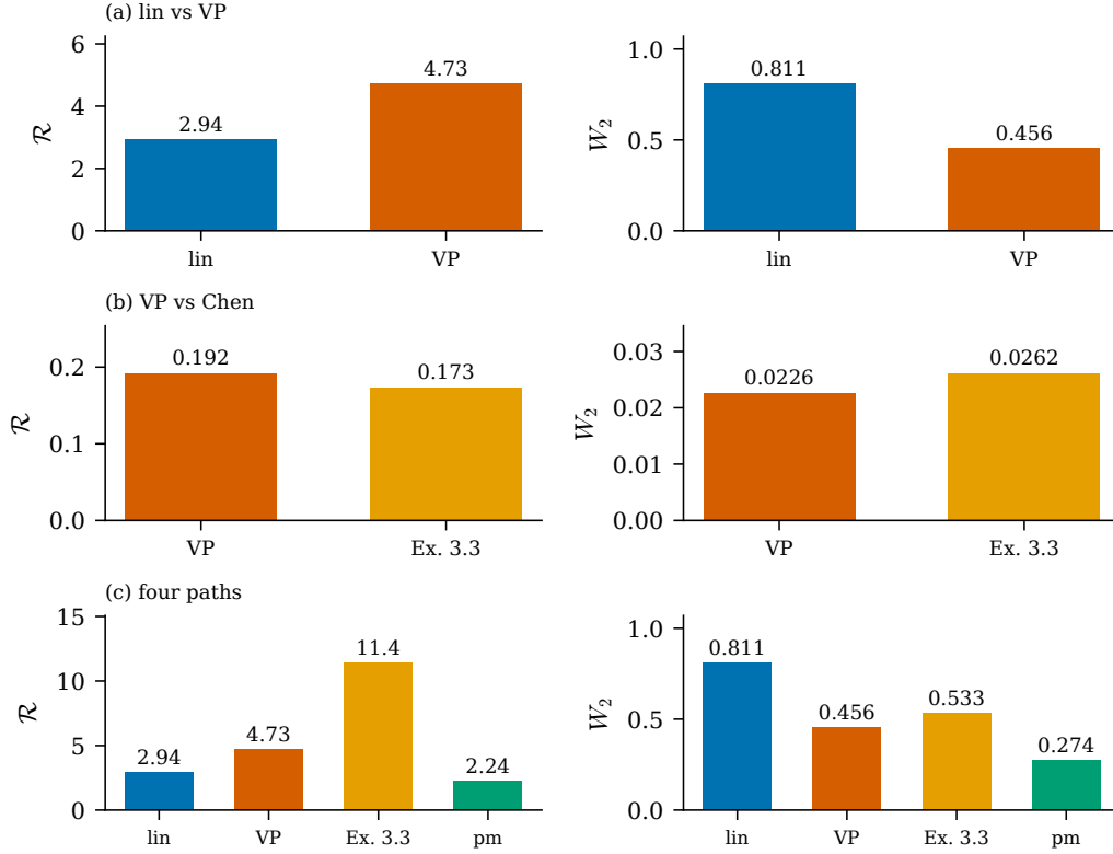
Figure 2: Three comparisons on commuting Gaussian interpolants. Continuous \mathcal{R} (left) and equal-NFE Gaussian W_2 (right). (a) Pairwise linear versus VP on rank-2 factor-plus-noise d = 8 , Euler, NFE 8. (b) VP versus Chen Ex. 3.3 scalar on anisotropic d = 8 , Euler, NFE 8. (c) Four specified candidate paths on rank-2 factor-plus-noise d = 8 , Euler, NFE 8. Among those four paths, the per-mode path has the smallest \mathcal{R} and the smallest W_2 in 36 of 36 tested blocks.
