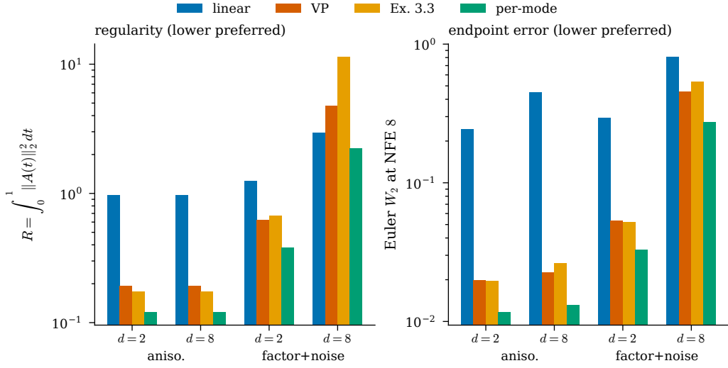
Figure 3: Four specified candidate paths on the four centered geometries. Left: continuous \mathcal{R} . Right: Euler Gaussian W_2 at NFE 8.
