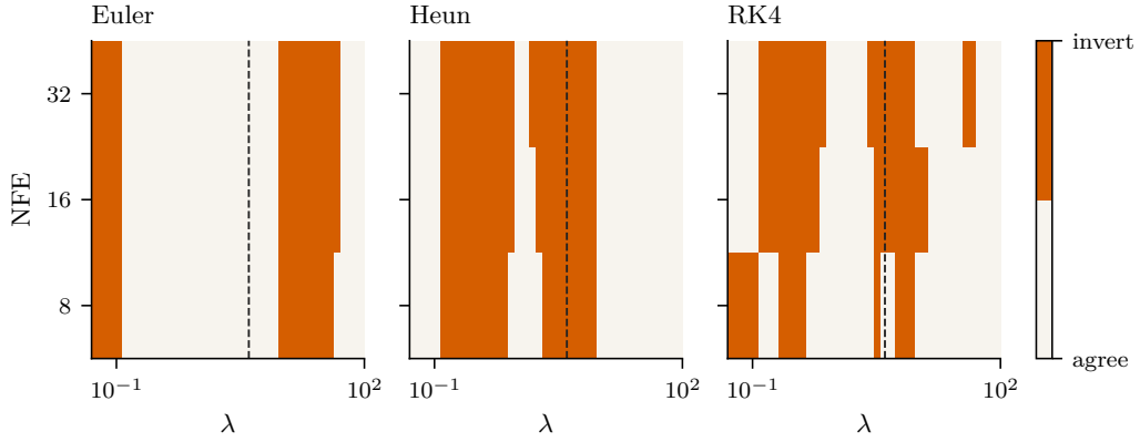
Figure 4: Linear versus VP ranking inversion versus target variance \lambda . Dark cells: \mathcal{R} and W_2 disagree. The dashed line is \lambda = 4 (Proposition 2).
