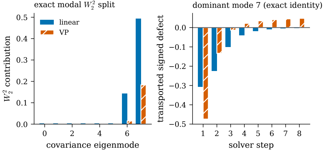
Figure 5: Modal contributions to squared Wasserstein error and transported signed defects for the strongest centered inversion. The bars reconstruct the telescoping identity (13). Exact modal identity on one block; illustration, not an independent causal test.
