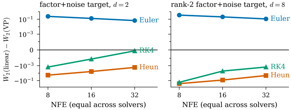
Figure 6: Signed factor-plus-noise W_2 margin at equal NFE. Positive values prefer VP; negative values prefer linear. Vertical axis: symmetric-log with linear threshold 10^{-4} . Exact-moment modal Runge–Kutta.
