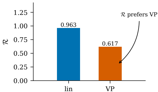
(b) exact \mathcal{R}
