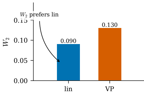
(c) Heun W_2
