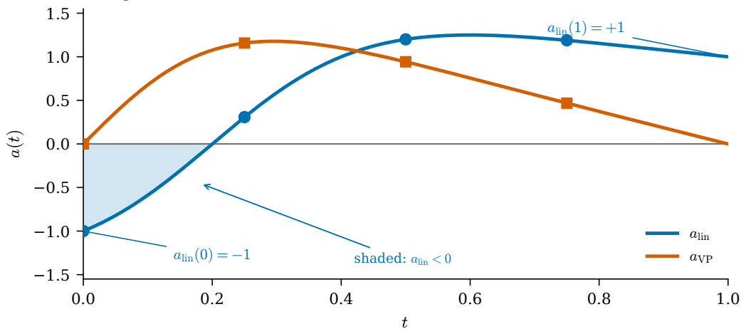
(b) exact \mathcal{R}
