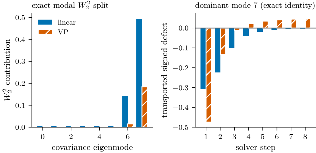
Figure 5: Modal contributions to squared Wasserstein error and transported signed defects for the strongest centered inversion. The bars reconstruct the telescoping identity (11). Exact modal identity on one block; illustration, not an independent causal test.
