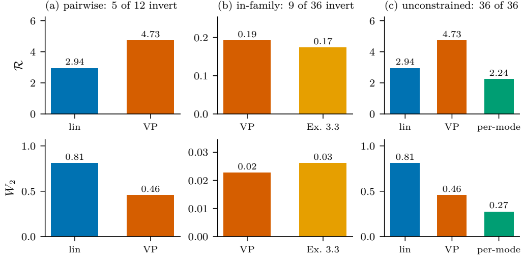
Figure 1: Three regimes for \mathcal{R} on commuting Gaussian interpolants. Each panel shows continuous \mathcal{R} and equal-NFE Gaussian W_2 (lower is preferred). (a) Pairwise linear versus VP on low-rank d = 8 , Euler, NFE 8: \mathcal{R} and W_2 invert; this occurs in 5 of 12 geometry \times solver cells. (b) In-family VP versus shared Chen Ex. 3.3 scalar ( M = \lambda_{\max} ) on anisotropic d = 8 , Euler, NFE 8: inversion, as in 9 of 36 blocks. (c) Unconstrained per-mode q_i(t) = \lambda_i^t on the same block: smallest \mathcal{R} and smallest W_2 in 36 of 36 blocks; not a shared (\alpha, \sigma) interpolant for d \geq 2 . Exact-moment modal Runge–Kutta; census counts, not estimators.
