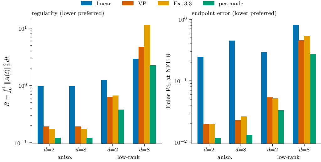
Figure 3: Four paths on the four centered geometries: linear, trigonometric VP, shared Chen Example 3.3 scalar schedule with M = \lambda_{\max} , and the unconstrained per-mode log-covariance schedule. Left: continuous \mathcal{R} . Right: Euler Gaussian W_2 at NFE 8. The per-mode schedule is not a shared (\alpha, \sigma) interpolant for d \geq 2 . Exact-moment modal Runge–Kutta; \mathcal{R} by adaptive quadrature except the per-mode closed form.
