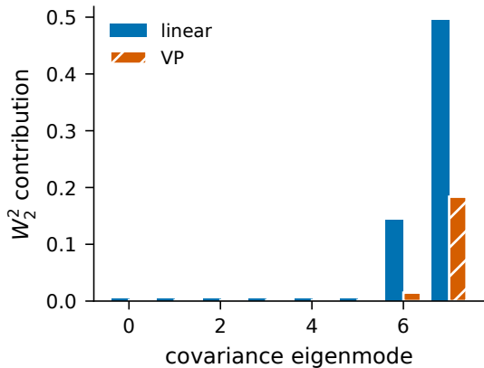
exact modal W_2^2 split
