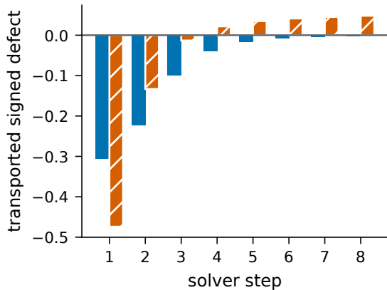
dominant mode 7 (exact identity)
