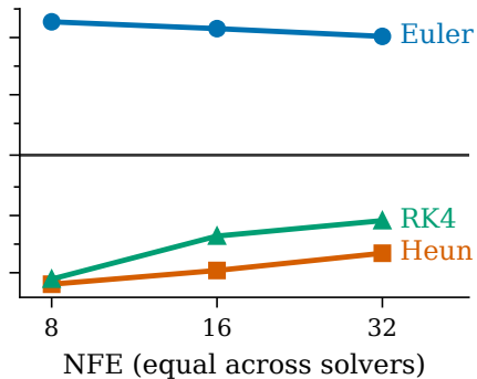
low-rank target, d = 8
