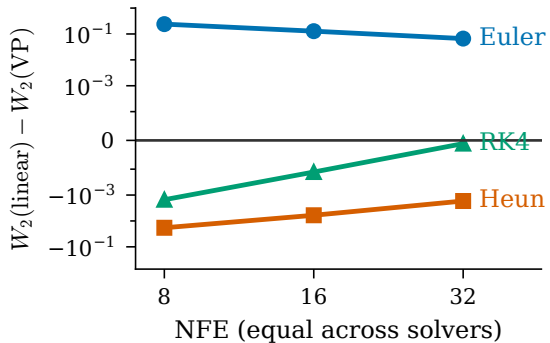
low-rank target, d = 2
