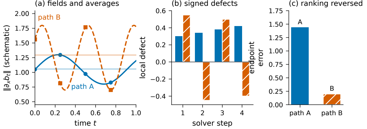
Figure 1: Conceptual schematic, not experimental data. (a) Averaging collapses two time-dependent fields to two scalars, while a solver samples only stage locations (markers). (b) Local defects are signed: same-sign defects accumulate, alternating defects cancel. (c) After transport to the endpoint, the error ranking can oppose the averaged ranking. The panel illustrates the accounting of Section 5, not the measured mechanism of any specific Gaussian inversion.
