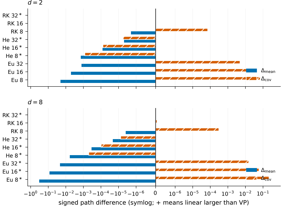
Figure 5: Signed path differences on all 18 non-centered blocks. \Delta_{\text{mean}} = M_{\text{lin}} - M_{\text{VP}} and \Delta_{\text{cov}} = C_{\text{lin}} - C_{\text{VP}} . A positive bar means the linear path has the larger contribution; a negative bar means VP has the larger contribution. The axis is symmetric-log with linear threshold 10^{-6} . Stars mark ranking inversions. Exact numerical values appear in Table 4.
