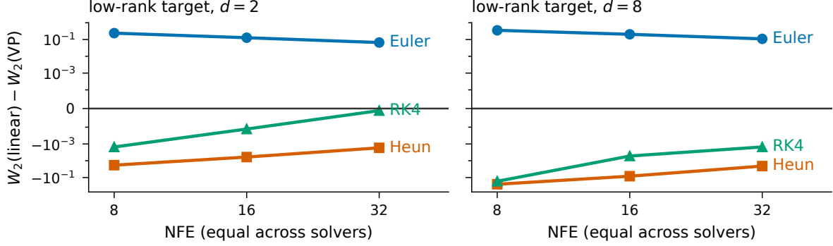
Figure 4: Signed low-rank W_2 margin at equal NFE. Positive values prefer VP; negative values prefer linear. Vertical axis: symmetric-log with linear threshold 10^{-4} .
