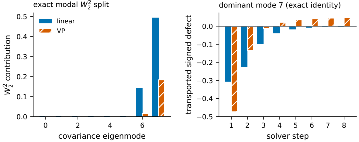
Figure 2: Modal contributions to squared Wasserstein error and transported signed defects for the strongest centered inversion. The bars reconstruct the telescoping identity (11).
