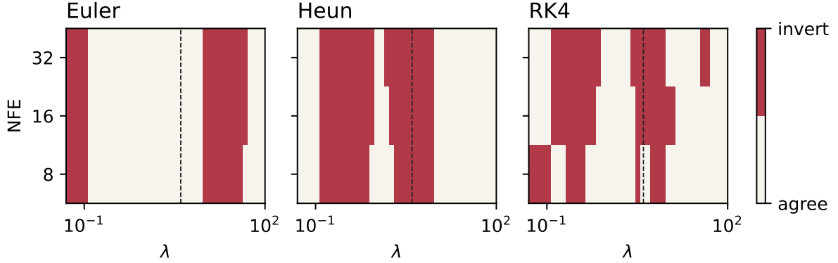
Figure 3: Linear versus VP ranking inversion versus target variance \lambda . Dark cells: \mathcal{R} and W_2 disagree. The dashed line is \lambda = 4 (Proposition 1).
