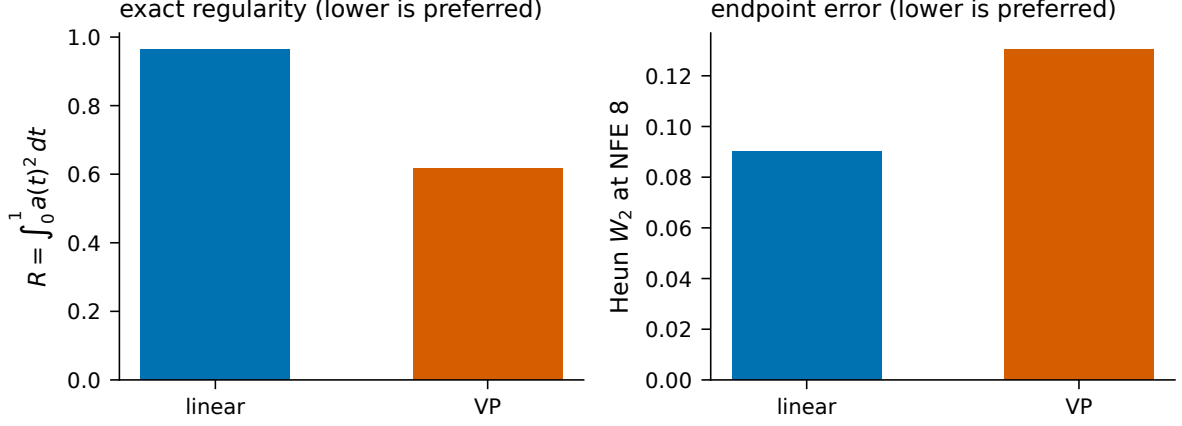
Figure 1: Proposition 1: exact \mathcal{R} (left) and Heun W_2 at NFE 8 (right). The VP error bar is the certified lower bound 2 - P(355/113, 99/70) . Regularity prefers VP; endpoint error prefers linear.
