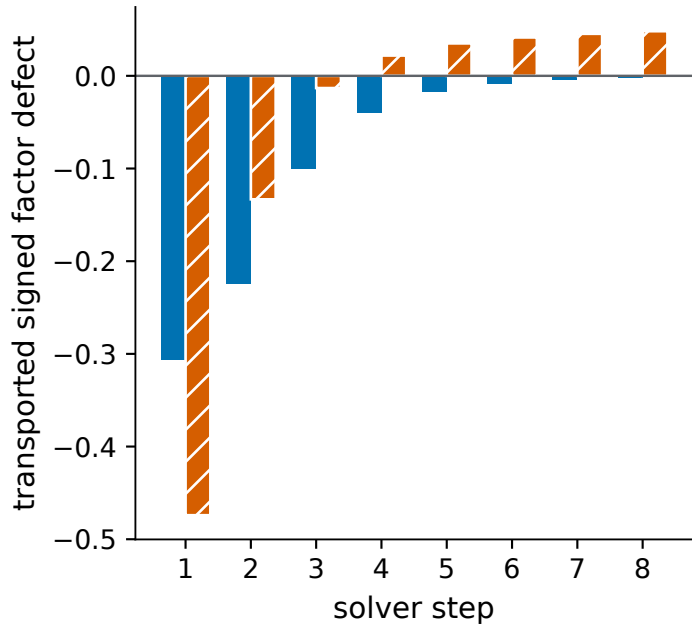
dominant mode 7 (exact identity)
