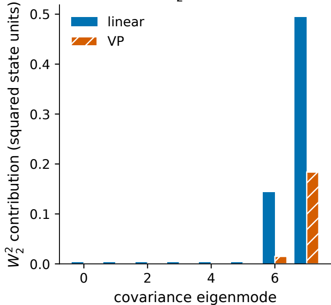
exact modal W_2^2 split
