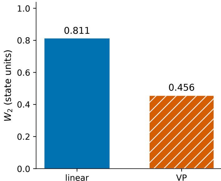
endpoint Gaussian W_2
