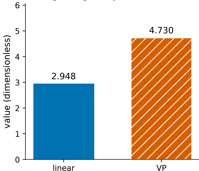
averaged regularity \mathcal{R}[b]
