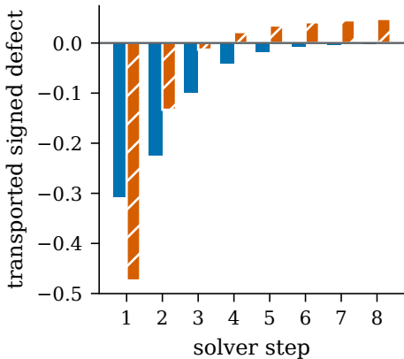
dominant mode 7 (exact identity)
