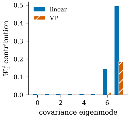
exact modal W_2^2 split
