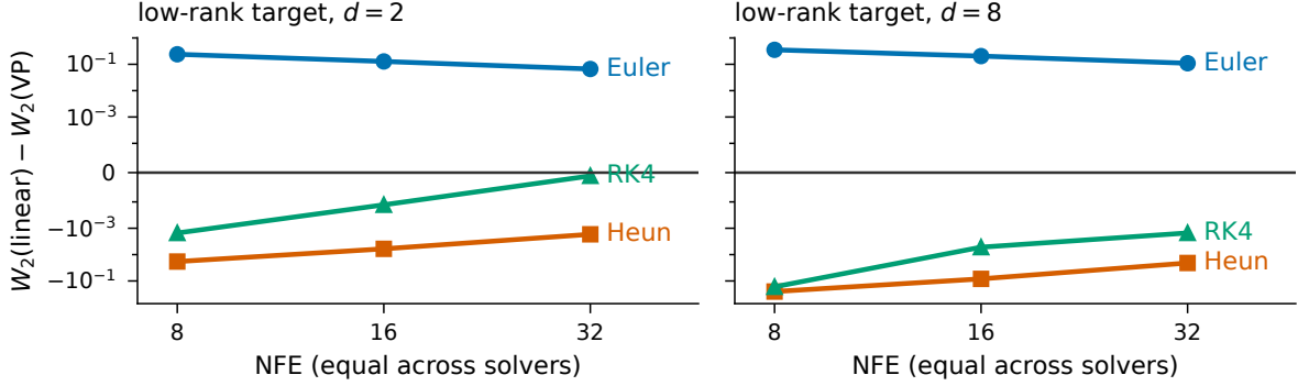
Figure 6: Signed low-rank W_2 margin at equal NFE. Positive values prefer VP; negative values prefer linear. Vertical axis: symmetric-log with linear threshold 10^{-4} . Exact-moment modal Runge–Kutta.
