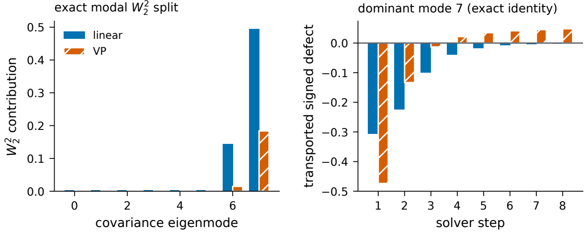
Figure 5: Modal contributions to squared Wasserstein error and transported signed defects for the strongest centered inversion. The bars reconstruct the telescoping identity (12). Exact modal identity on one block; illustration, not an independent causal test.
