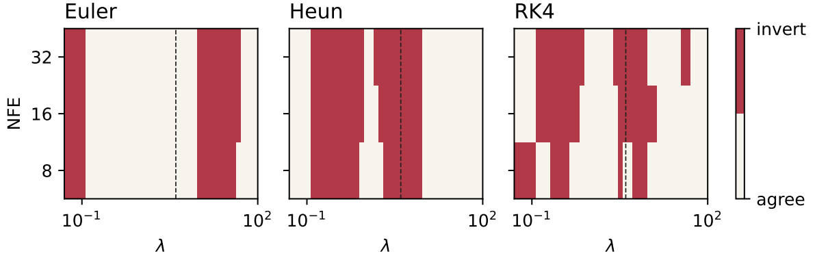
Figure 4: Linear versus VP ranking inversion versus target variance \lambda , for Euler, Heun, and RK4 at NFE 8, 16, and 32. Dark cells: \mathcal{R} and W_2 disagree. The dashed line is \lambda = 4 (Proposition 2). The inversion set is reported in the text by its Lebesgue measure in \log \lambda on [0.05, 100] , not by a count of dark pixels. Numerical evaluation of a deterministic ranking.
