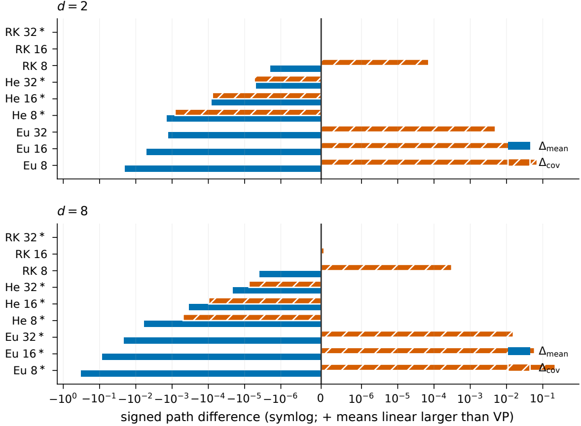
Figure 7: Signed path differences on all 18 non-centered blocks. \Delta_{\text{mean}} = M_{\text{lin}} - M_{\text{VP}} and \Delta_{\text{cov}} = C_{\text{lin}} - C_{\text{VP}} . A positive bar means the linear path has the larger contribution; a negative bar means VP has the larger contribution. The axis is symmetric-log with linear threshold 10^{-6} . Stars mark ranking inversions. Exact numerical values appear in Table 9.
