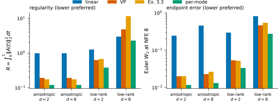
Figure 3: Four paths on the four centered geometries: linear, trigonometric VP, shared Chen Example 3.3 scalar schedule with M = \lambda_{\max} , and the unconstrained per-mode log-covariance schedule. Left: continuous \mathcal{R} . Right: Euler Gaussian W_2 at NFE 8. The per-mode schedule is not a shared (\alpha, \sigma) interpolant for d \geq 2 . Exact-moment modal Runge–Kutta; \mathcal{R} by adaptive quadrature except the per-mode closed form.
