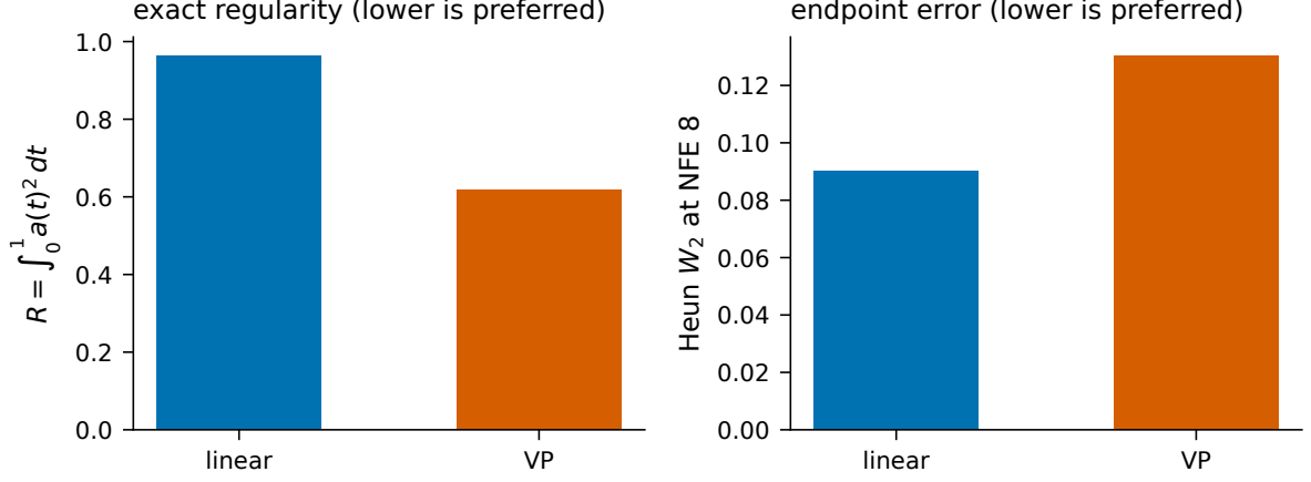
Figure 2: Proposition 2: exact \mathcal{R} (left) and Heun W_2 at NFE 8 (right). The right-hand VP bar is the certified lower bound 2 - P(355/113, 99/70) , not a statistical interval. Regularity prefers VP; endpoint error prefers linear. Exact calculation.
