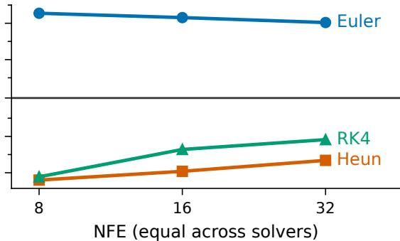
low-rank target, d = 8
