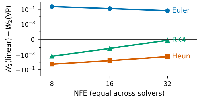
low-rank target, d = 2
