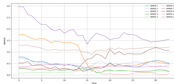
Figure 2.25: Evolution of the NRMSEs over EnKF analysis phases
