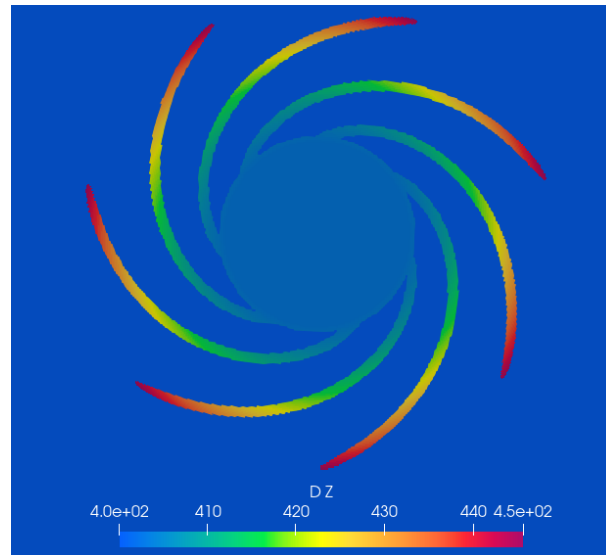
Figure 2.26: Radial expansion of Dz over the impeller radius
