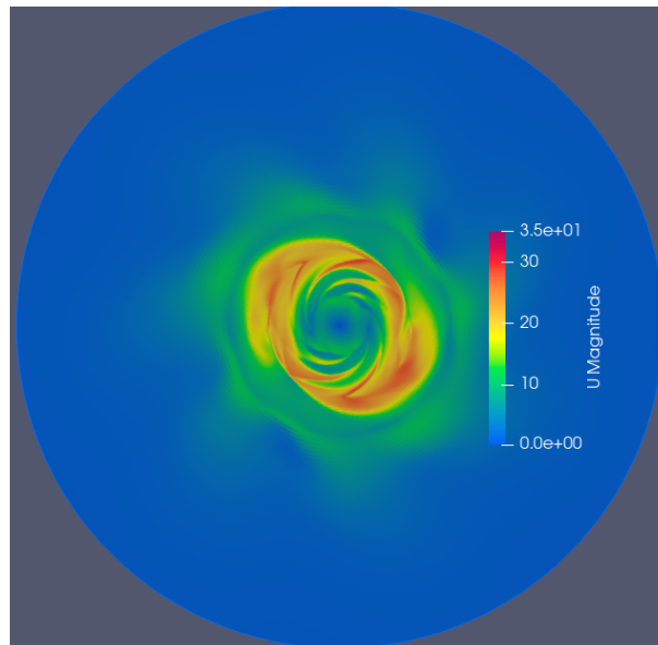
Figure 2.24: Velocity field for Dx = 4e7 and Dy = 2e7
