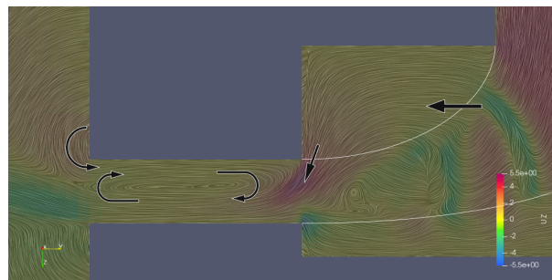
Figure 2.27: Formation of the recirculation bubble in the diffuser
