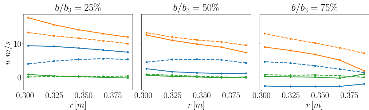
Figure 2.21: Comparison between the profiles inside the diffuser for the numerical simulation (continuous lines), and the PIV data (dashed lines). In particular, (—) represents the radial velocity u_r , (—) depicts the azimuthal velocity u_\theta , and (—) illustrates the vertical velocity u_z .
