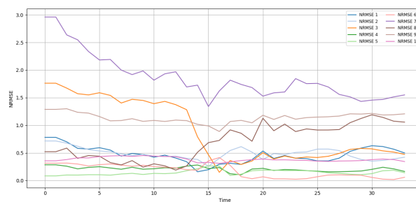
Figure 2.18: Evolution of the NRMSEs over EnKF analysis phases
