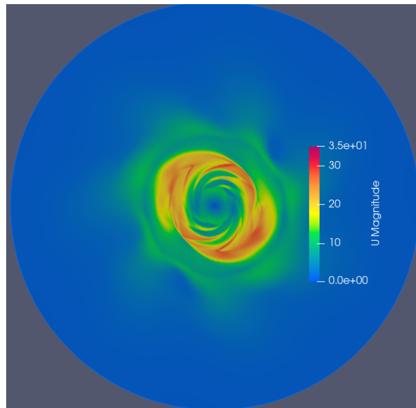
Figure 2.17: Velocity field for Dx = 4e7 and Dy = 2e7
