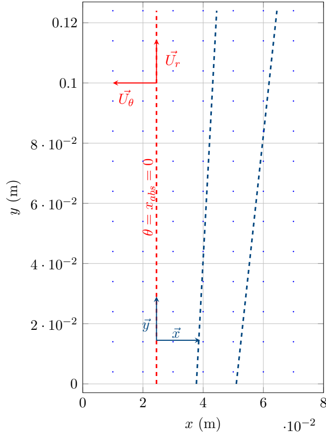
Figure 3.6: PIV acquisition zone in the RESEDA experiment, with orientation of the (r, \theta) velocity components.
