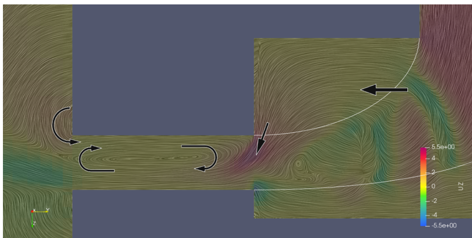
Figure 3.13: Formation of the recirculation bubble in the diffuser
