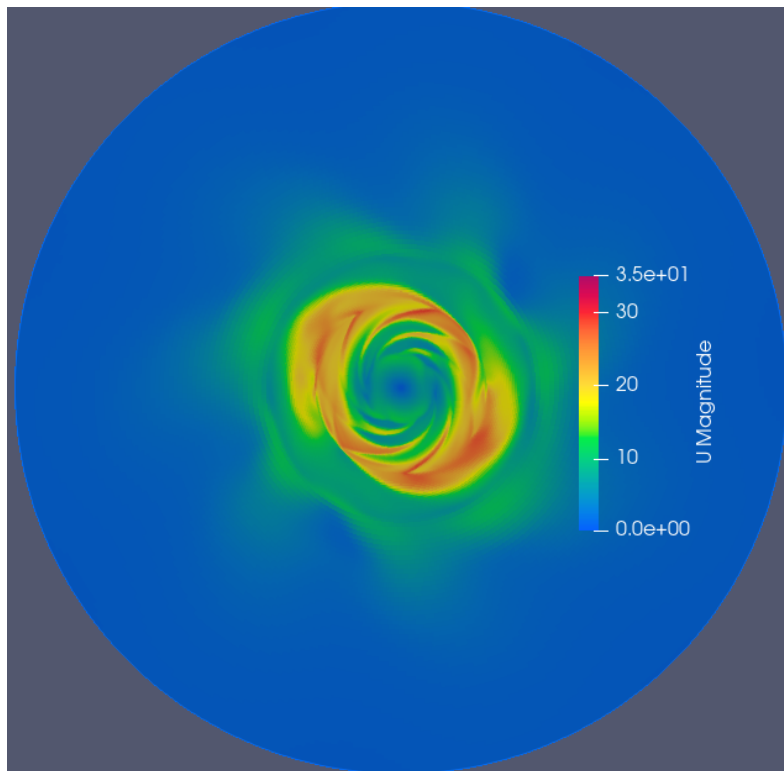
Figure 3.12: First results of CONES optimisation. Slice at z = 0 , with \mathbf{D} = (4e7, 2e7, 4e7) , D_k = 3e7 and D_\omega = -3e7
