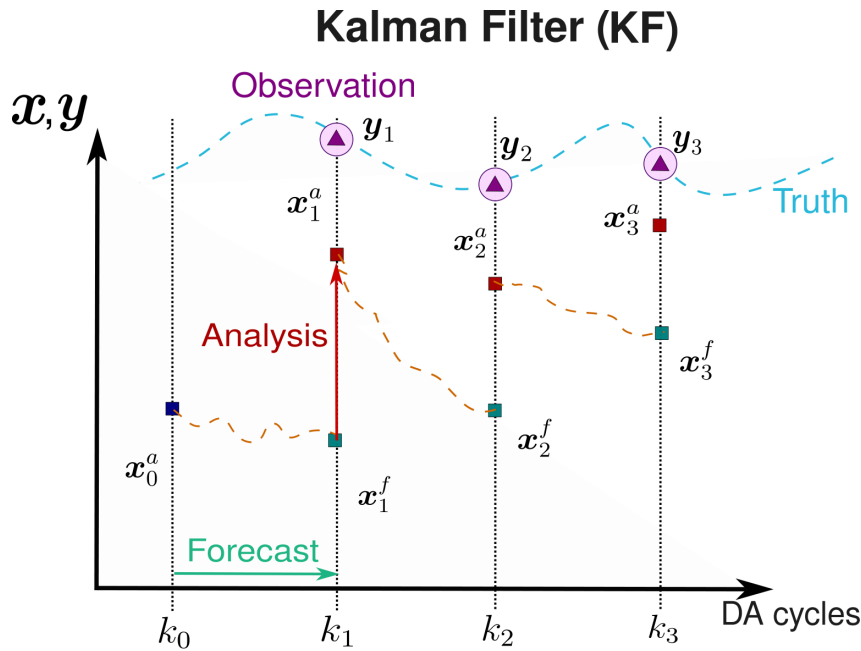
Figure 2.10: Kalman Filter process illustration
