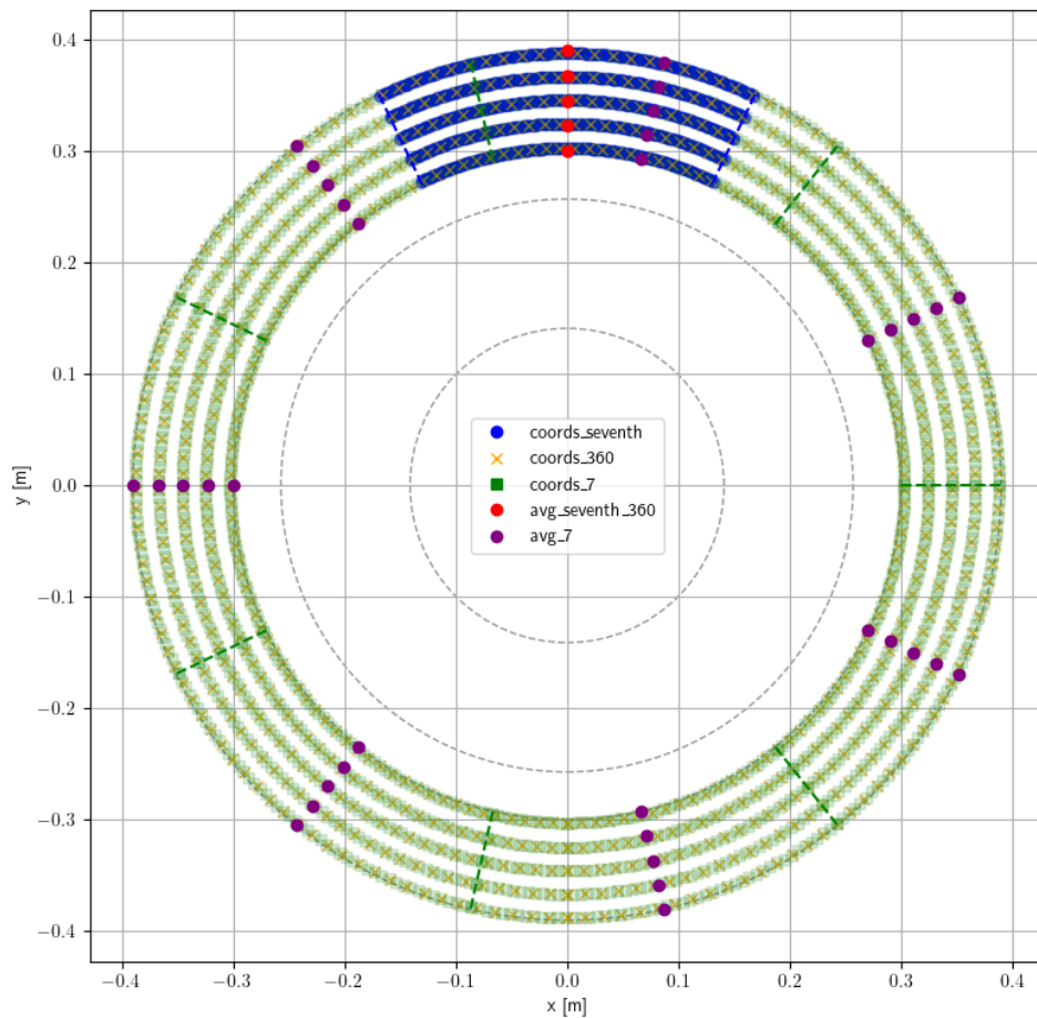
Figure 3.17: Illustration of the augmented coordinates for the interpolation of the field
