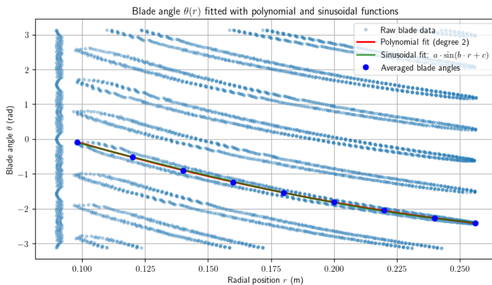
Figure 3.15: Polynomial and sinusoidal interpolation of the blade shape
