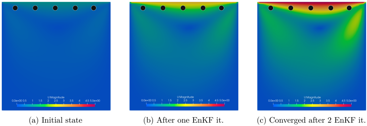
Figure 2.11: Evolution of the state through EnKF iterations (●: observation point)
