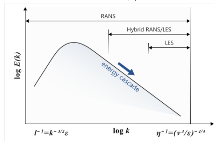
Figure 2.6: Turbulence models
