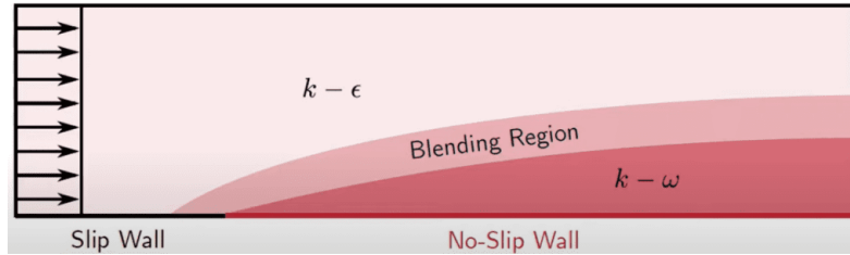
Figure 2.7: k - \omega SST model
