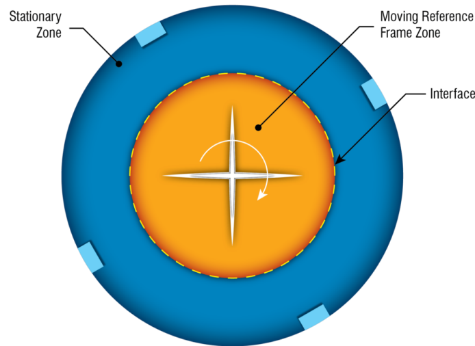
Figure 2.8: MRF strategy
