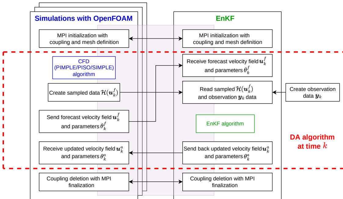
Figure 2.12: CONES structure
