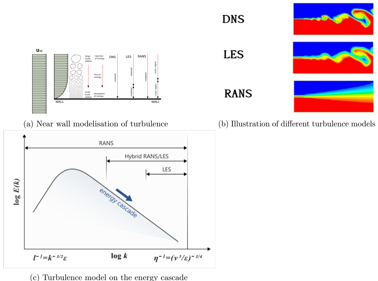
Figure 2.6: Turbulence models
