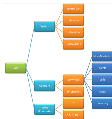
Figure 2.9: Tree of the OpenFOAM dictionaries
