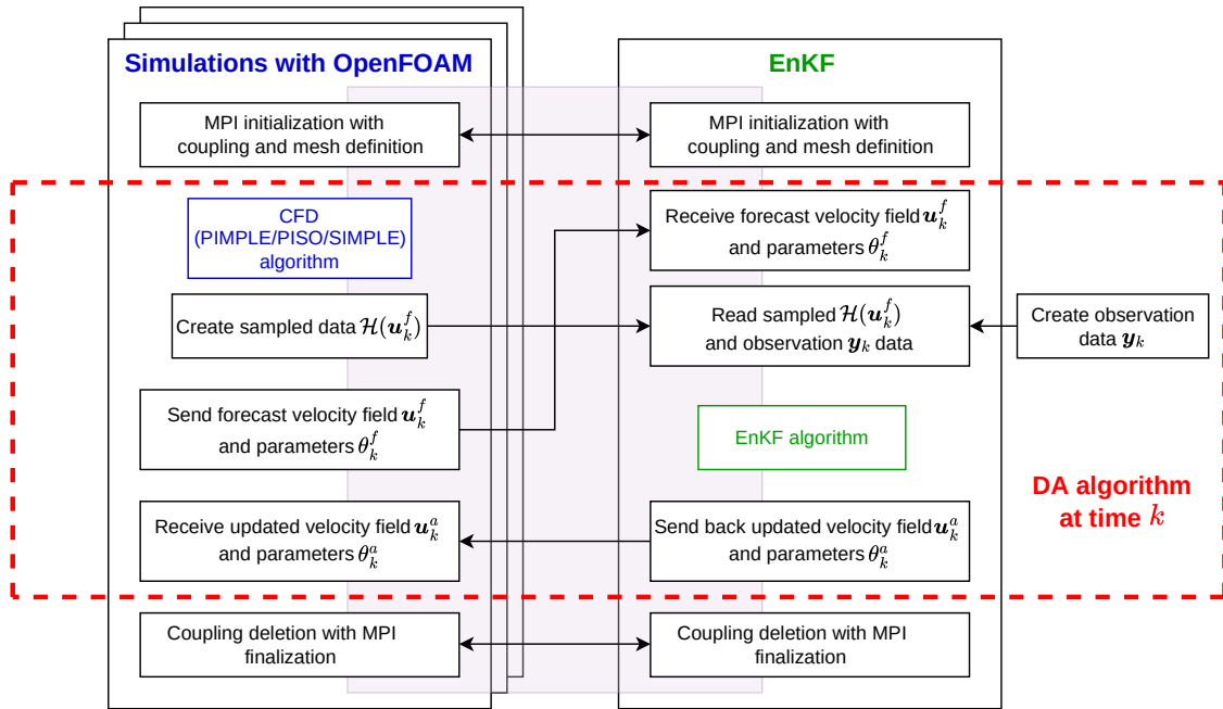
Figure 2.14: CONES structure
