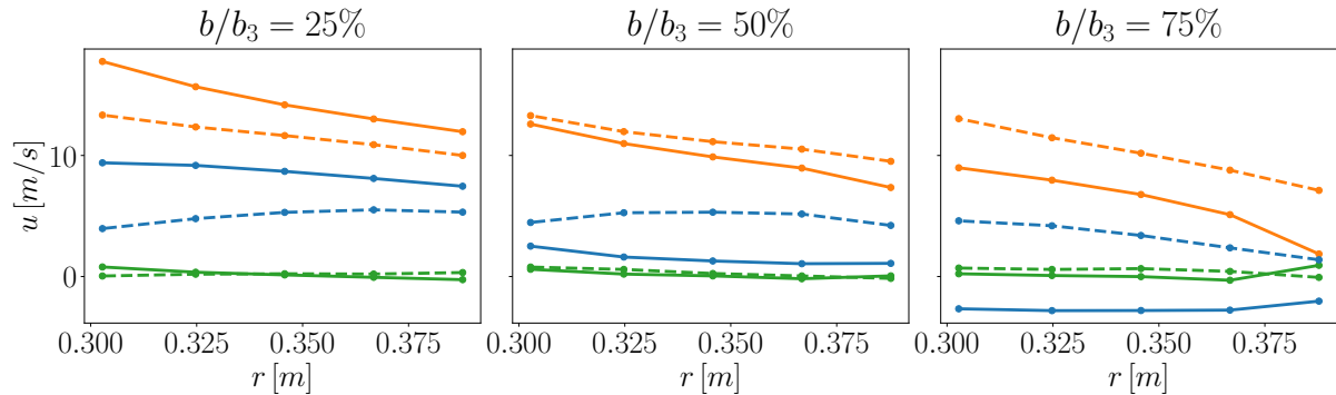
Figure 2.18: Comparison between the profiles inside the diffuser for the numerical simulation (continuous lines), and the PIV data (dashed lines). In particular, (—) represents the radial velocity u_r , (—) depicts the azimuthal velocity u_\theta , and (—) illustrates the vertical velocity u_z .
