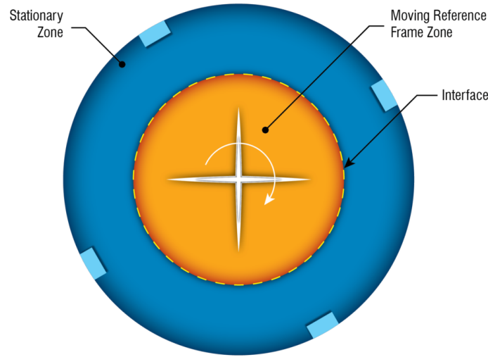
Figure 2.7: MRF strategy: the rotating region is solved in a non-inertial frame
