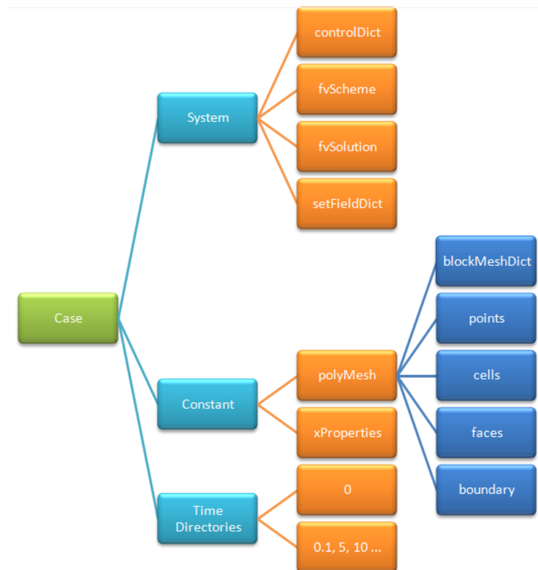
Figure 2.9: Tree of the OpenFOAM dictionaries
