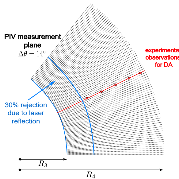
Figure 2.22: Position of the PIV points on a polar slice of the diffuser
