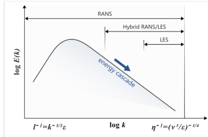
Figure 2.5: Turbulence models
