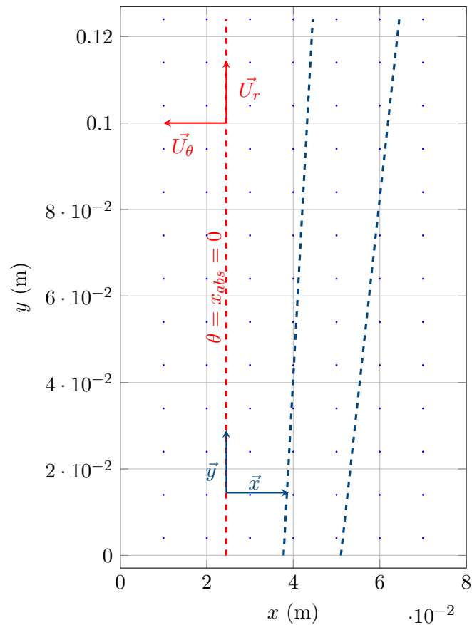
Zone d'acquisition PIV
