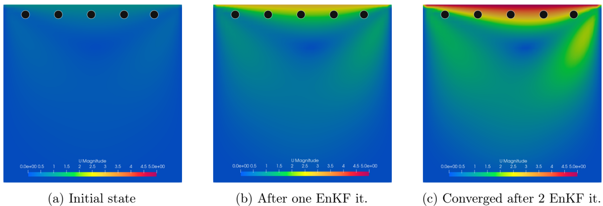
Figure 2.13: Evolution of the state through EnKF iterations (●: observation point)
