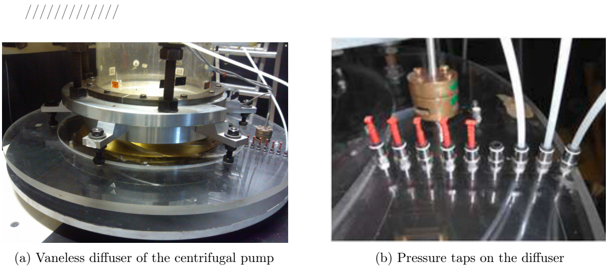
Figure 2.20: Diffuser and pressure taps of the centrifugal pump
