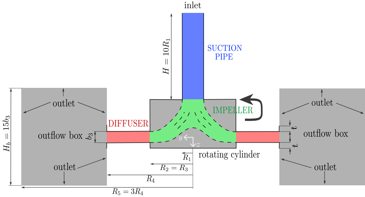
Figure 2.15: Model of the RESEDA benchmark
