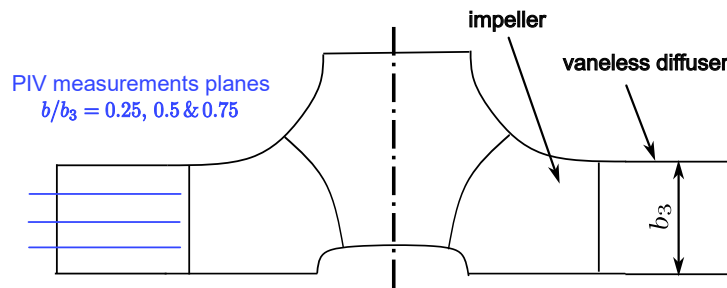
Figure 2.20: Position of the PIV planes on the diffuser
