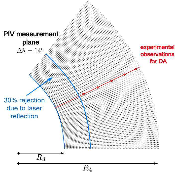
(b) Position of the PIV points on a polar slice of the diffuser
