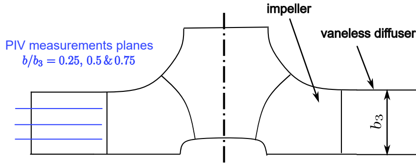
(a) Position of the PIV plans on the diffuser
