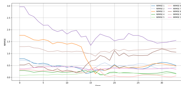
Figure 2.30: Evolution of the NRMSEs over EnKF analysis phases
