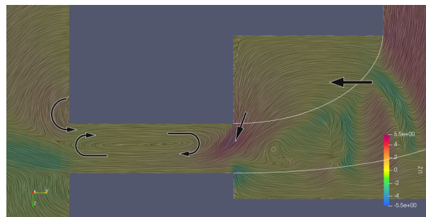
Figure 2.32: Formation of the recirculation bubble in the diffuser
