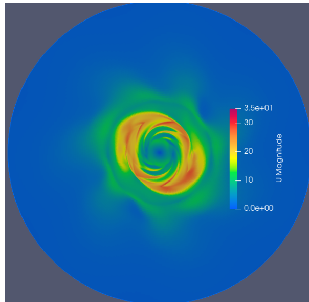
Figure 2.29: Velocity field for D_x = 4e7 and D_y = 2e7
