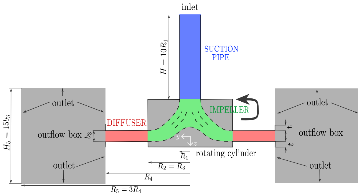
Figure 2.14: Model of the RESDA benchmark
