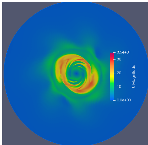
Figure 2.20: Velocity field for Dx = 4e7 and Dy = 2e7
