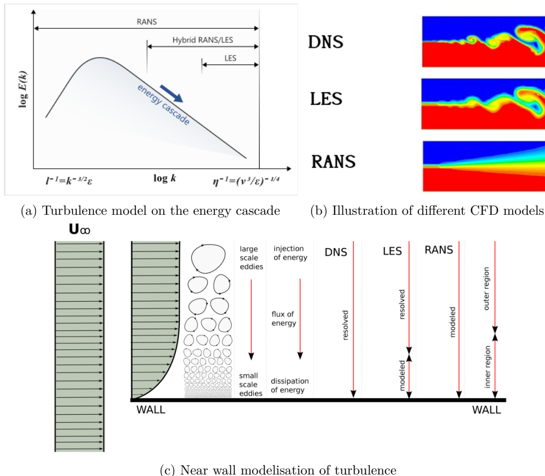
Figure 2.11: Turbulence models
