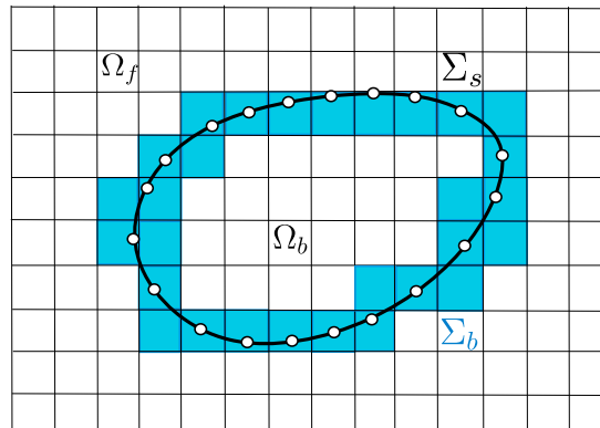
Figure 2.15: IBM regions
