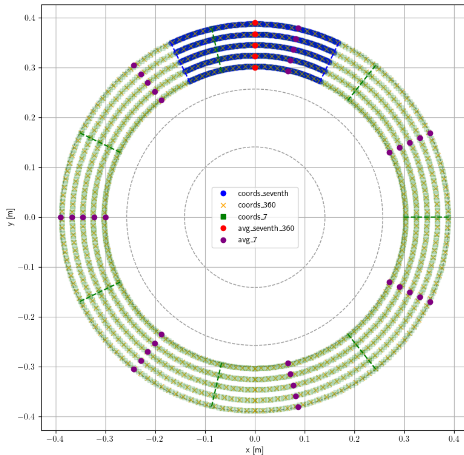
Figure 3.9: Illustration of the augmented coordinates for the interpolation of the field
