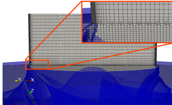
Figure 2.18: Mesh interface between the pipe and the impeller
