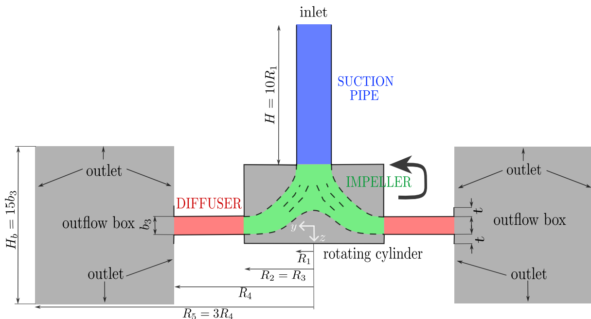
Figure 2.19: Model of the RESDA benchmark
