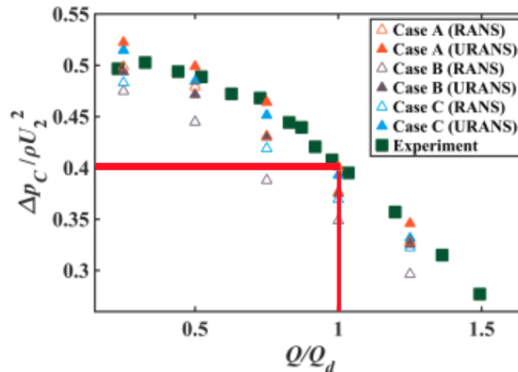
Figure 2.26: Overall pump performance versus reduced pump flow rate Q
