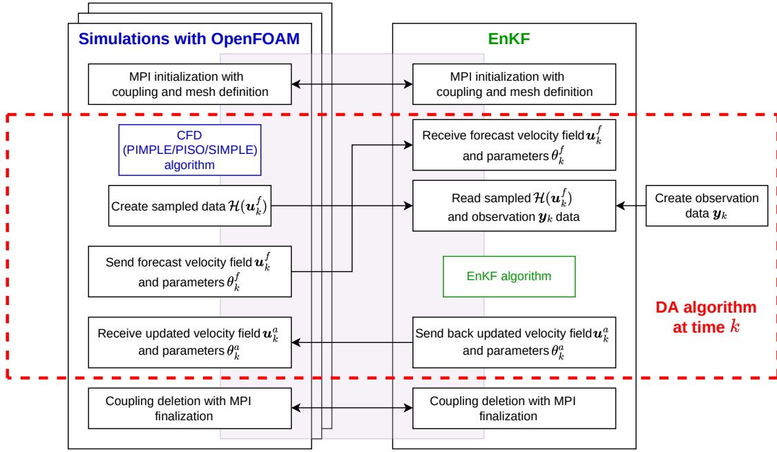
Figure 2.16: CONES structure
