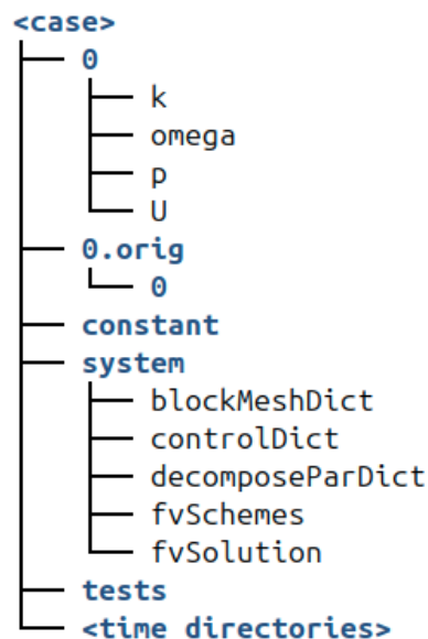
Figure 2.11: Tree of the OpenFOAM dictionaries
