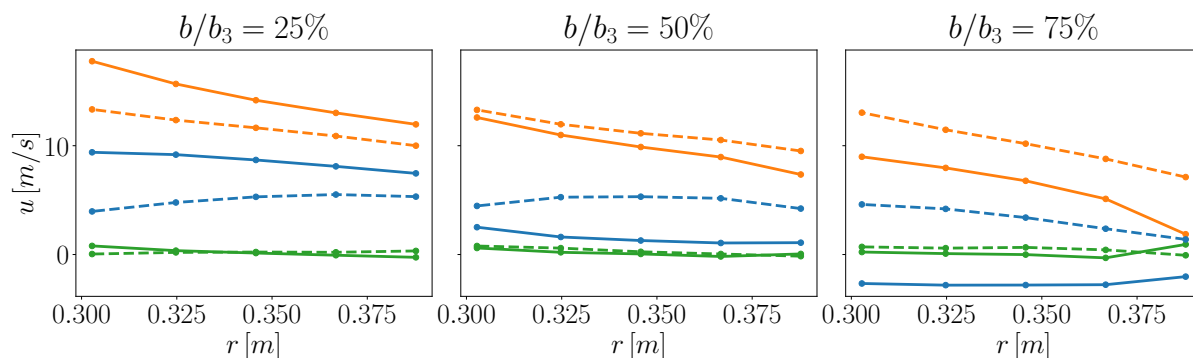
Figure 2.24: Comparison between the profiles inside the diffuser for the numerical simulation (continuous lines), and the PIV data (dashed lines). In particular, (—) represents the radial velocity u_r , (—) depicts the azimuthal velocity u_\theta , and (—) illustrates the vertical velocity u_z .
