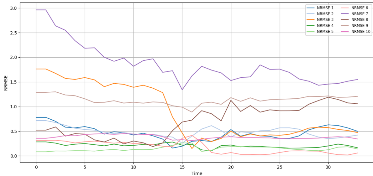
Figure 3.11: Evolution of the NRMSEs over EnKF analysis phases. Legend is organized as follows: NRMSE 1 to 3 are for the radial velocities at respectively 25%, 50% and 75% of the impeller height; NRMSE 4 to 6 for the azimuthal velocities and NRMSE 7 to 9 are ordered following the same ideal; NRMSE 10 is for the pressure difference between the inlet and the outlet of the pump.
