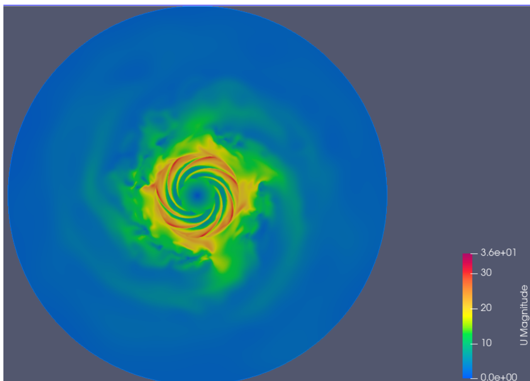
Figure 3.12: Velocity field for Dx = 4e7 and Dy = 2e7
