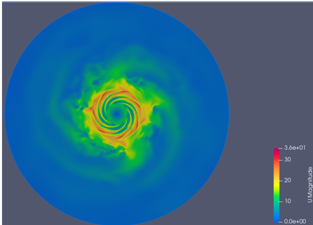
Figure 3.7: Velocity field for Dx = 4e7 and Dy = 2e7
