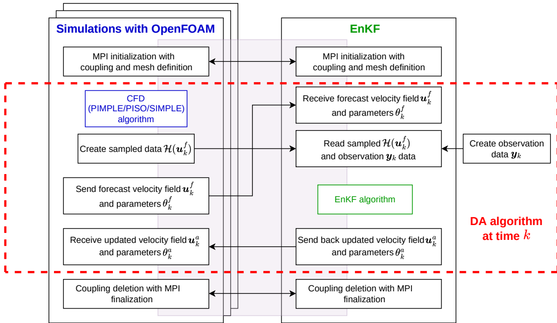
Figure 2.19: CONES structure
