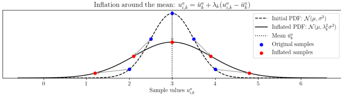
Figure 2.17: Deterministic inflation
