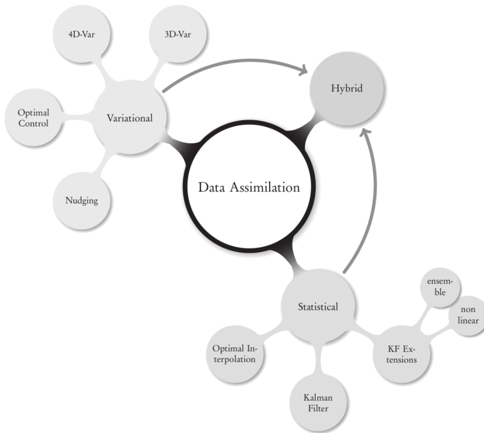
Figure 2.1: The big picture for DA methods and algorithms
