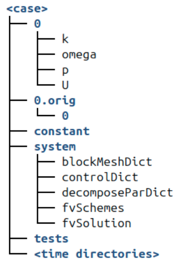
Figure 2.7: Arbo of OpenFoam
