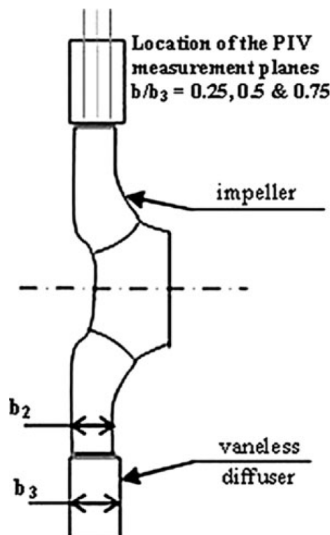
Figure 2.5: Position of the PIV plans
