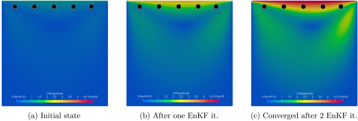
Figure 2.18: Evolution of the state through EnKF iterations (●: observation point)
