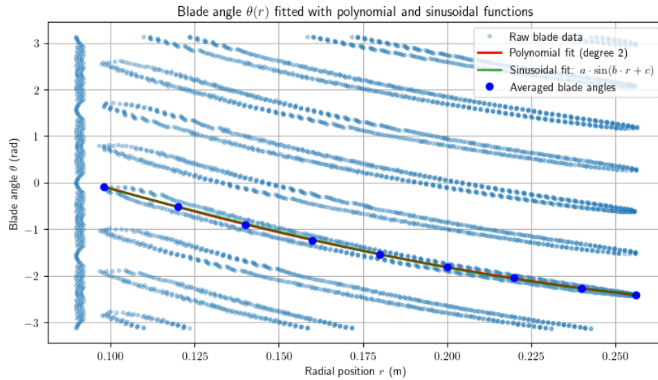
Figure 3.8: Polynomial and sinusoidal interpolation of the blade shape
