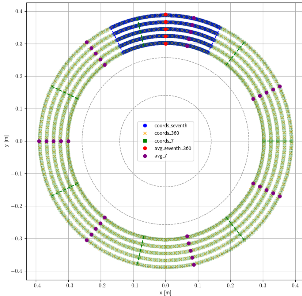
Figure 3.12: Illustration of the augmented coordinates for the interpolation of the field
