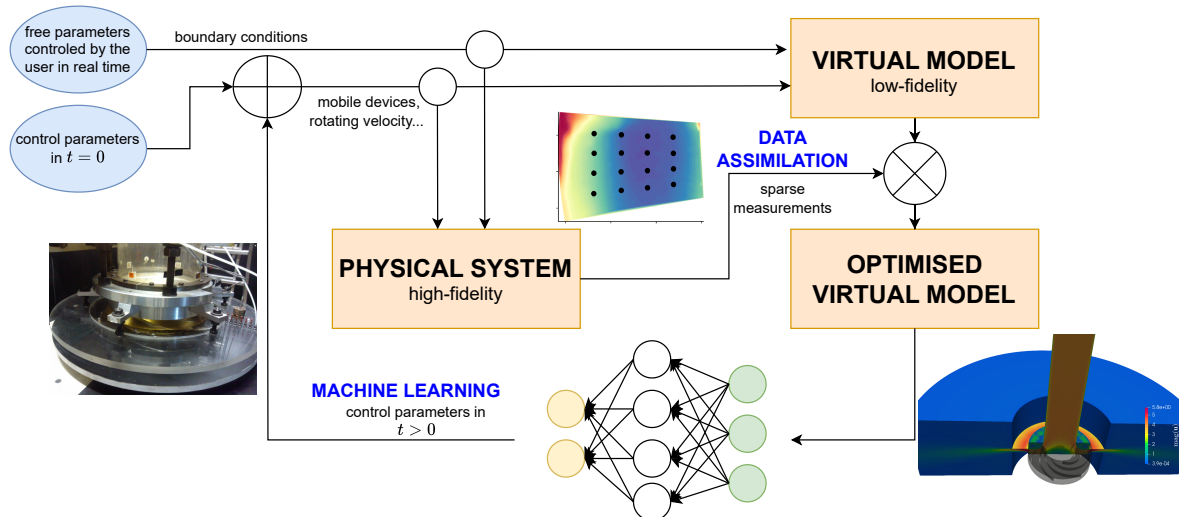
Figure 3.15: Illustration of a real-time Digital Twin framework for a centrifugal pump
