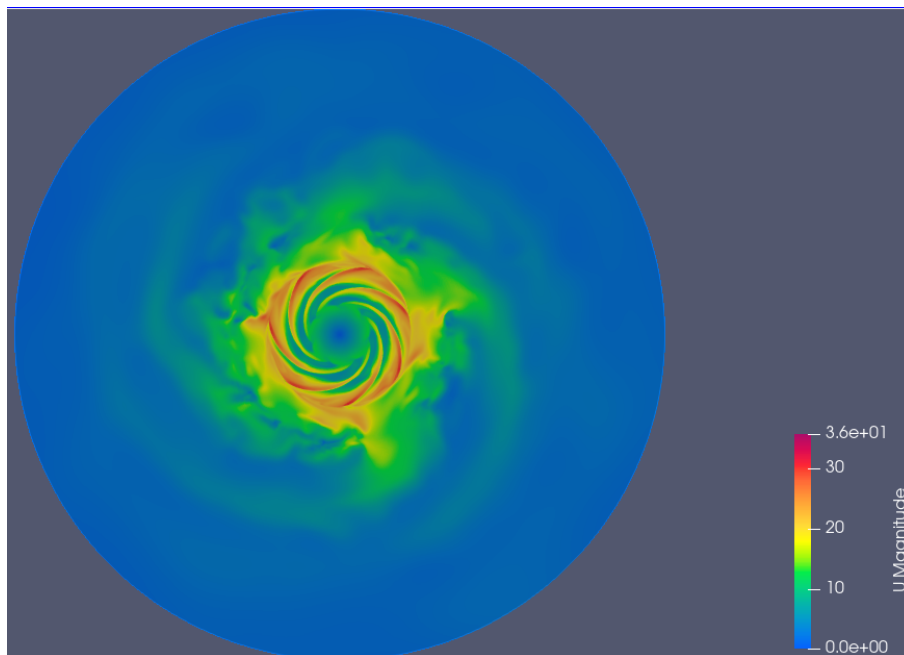
Figure 3.7: Velocity field for D_x = D_y , but with too high parameters, which made the simulation diverge
