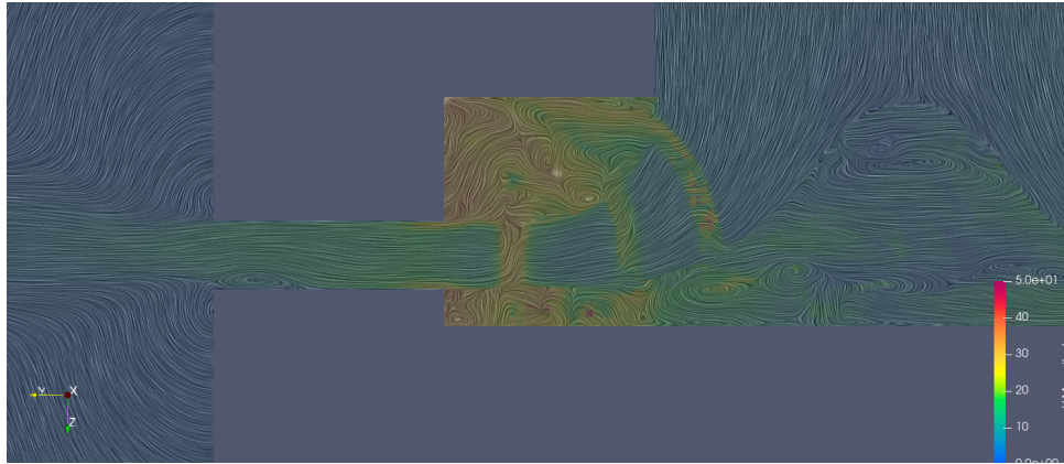
(b) Velocity field obtained a few iterations after enforcing \omega r .
