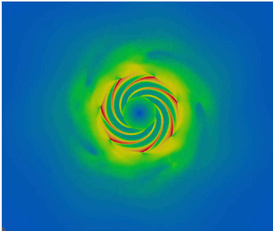
Figure 3.13: Velocity field diverged after applying all the strategies
