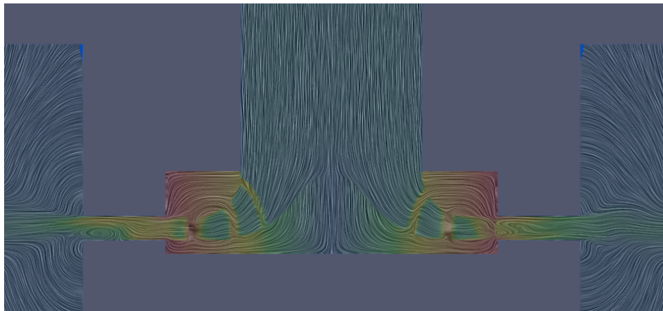
(c) Velocity field obtained long after enforcing \omega r , confirming the suppression of the recirculation bubble.
