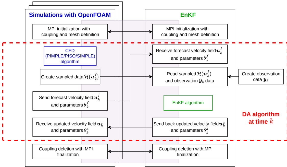
Figure 2.19: CONES structure
