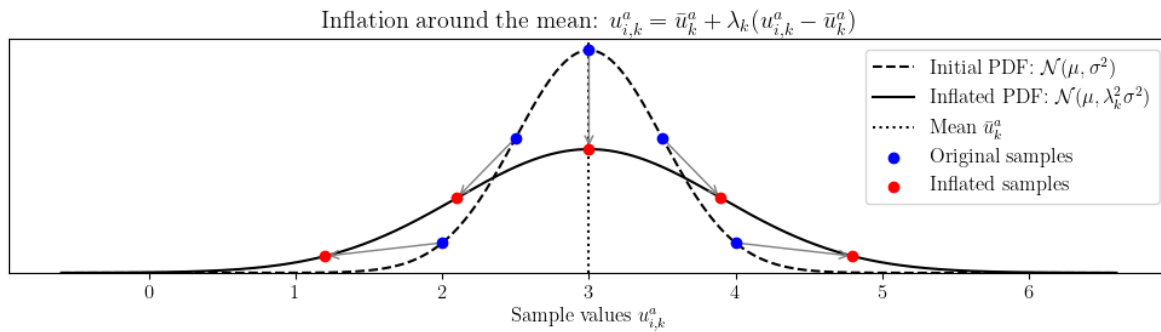
Figure 2.17: Deterministic inflation
