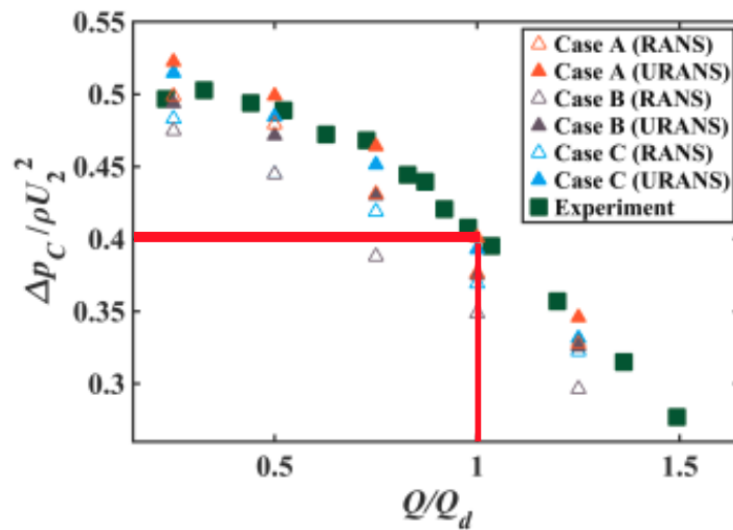
Figure 2.10: Overall pump performance versus reduced pump flow rate Q[4]
