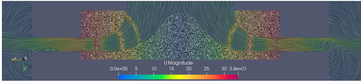
(a) Velocity field obtained by enforcing \omega r , showing an initial suppression of the recirculation bubble.
