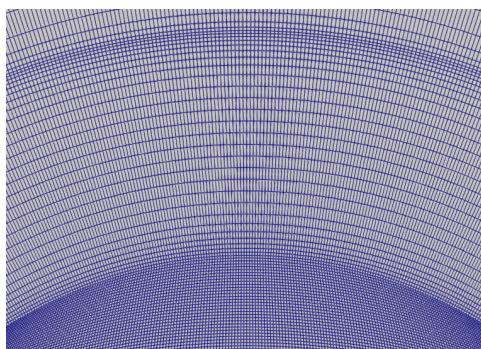
Figure 2.25: Diffuser Mesh
