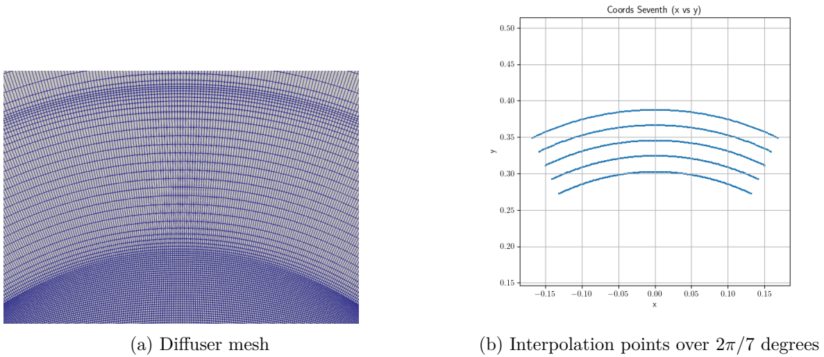
Figure 2.9: Diffuser mesh and interpolation points over 2\pi/7 degrees
