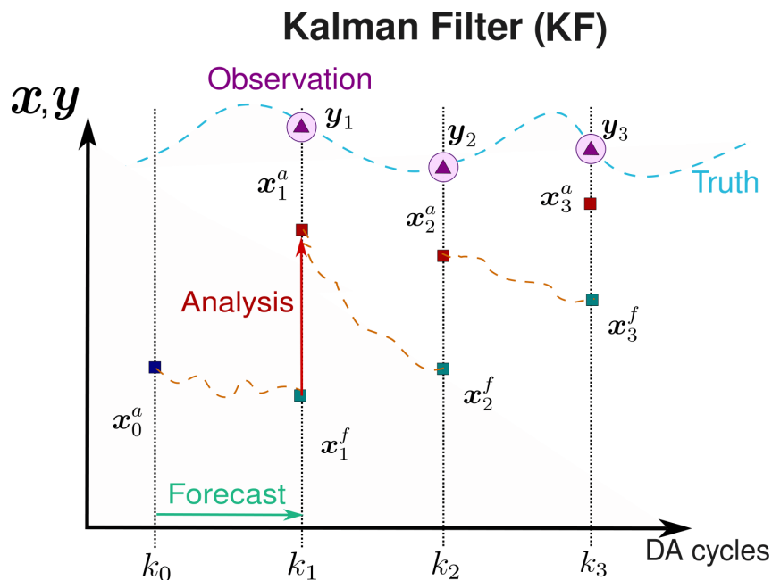
Figure 2.13: Kalman Filter process illustration
