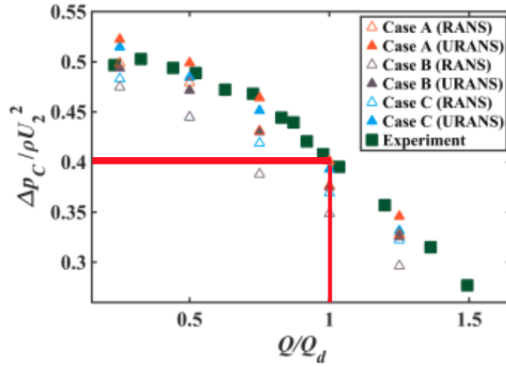
Figure 2.25: Overall pump performance versus reduced pump flow rate Q [4]
