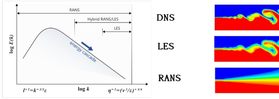
(b) Illustration of different CFD models
