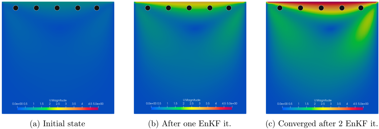
Figure 2.14: Evolution of the state through EnKF iterations (●: observation point)
