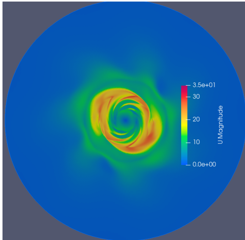
Figure 2.28: First results of CONES optimisation. Slice at z = 0
