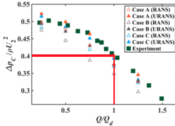
Figure 2.21: Overall pump performance versus reduced pump flow rate Q
