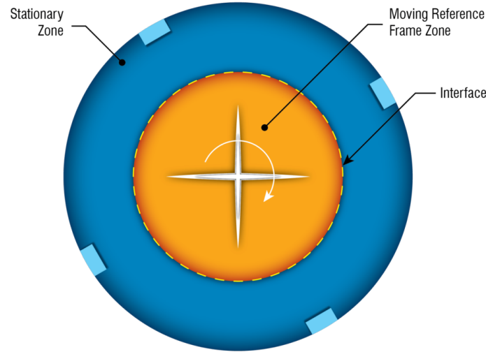
Figure 2.8: MRF strategy
