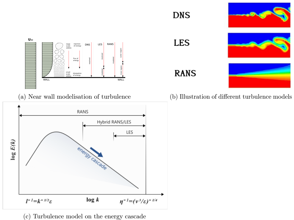
Figure 2.6: Turbulence models
