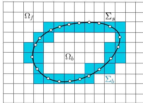
Figure 2.3: IBM regions
