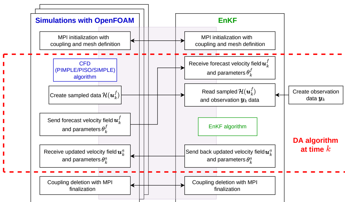
Figure 2.12: CONES structure
