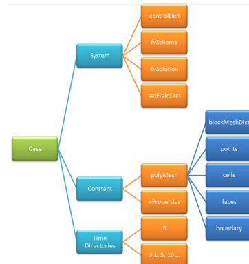
Figure 2.9: Tree of the OpenFOAM dictionaries
