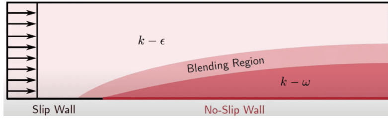
Figure 2.7: k - \omega SST model
