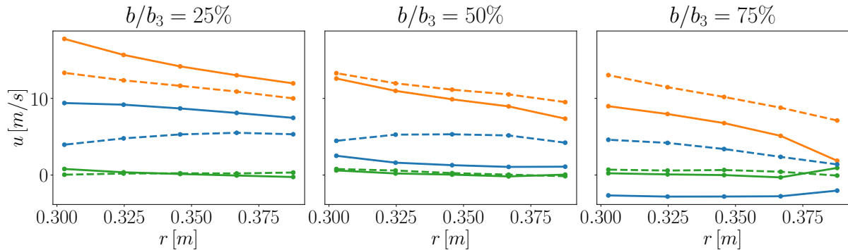
Figure 2.16: Comparison between the profiles inside the diffuser for the numerical simulation (continuous lines), and the PIV data (dashed lines). In particular, (—) represents the radial velocity u_r , (—) depicts the azimuthal velocity u_\theta , and (—) illustrates the vertical velocity u_z .
