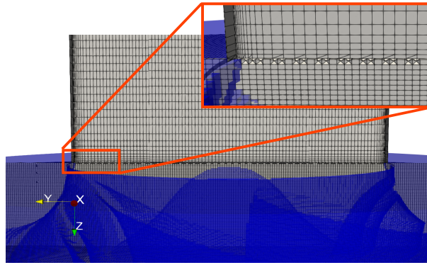
Figure 2.13: Mesh interface between the pipe and the impeller
