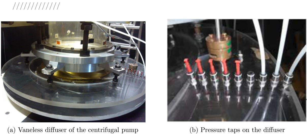
Figure 2.18: Diffuser and pressure taps of the centrifugal pump
