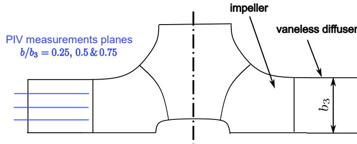
Figure 2.23: Position of the PIV planes on the diffuser
