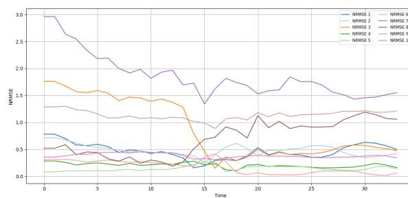
Figure 2.28: Evolution of the NRMSEs over EnKF analysis phases
