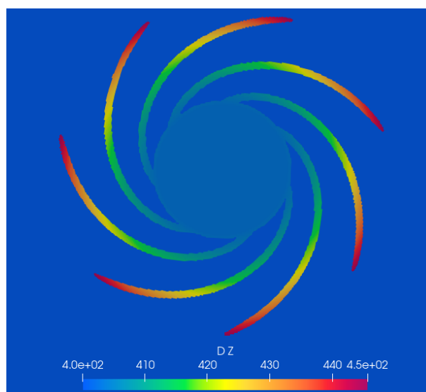
Figure 2.29: Radial expansion of Dz over the impeller radius
